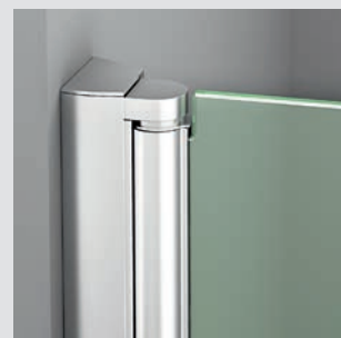
Detalle Cerco Vertical Pared
