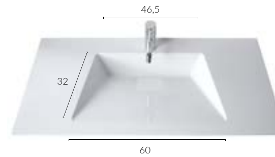
Centred washbasin ↗ 46 cm Poza centrada ↗ 46 cm Vasque centrée ↗ 46 cm
